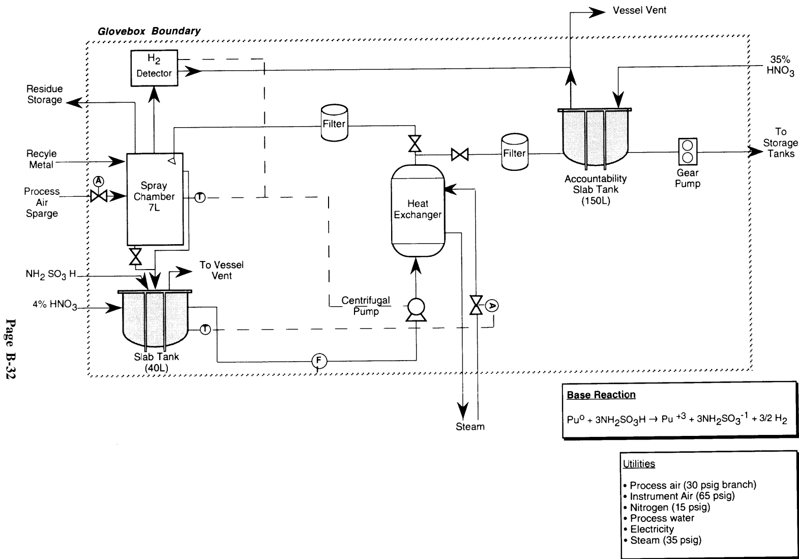
Figure B.8. Metal Dissolution Line
