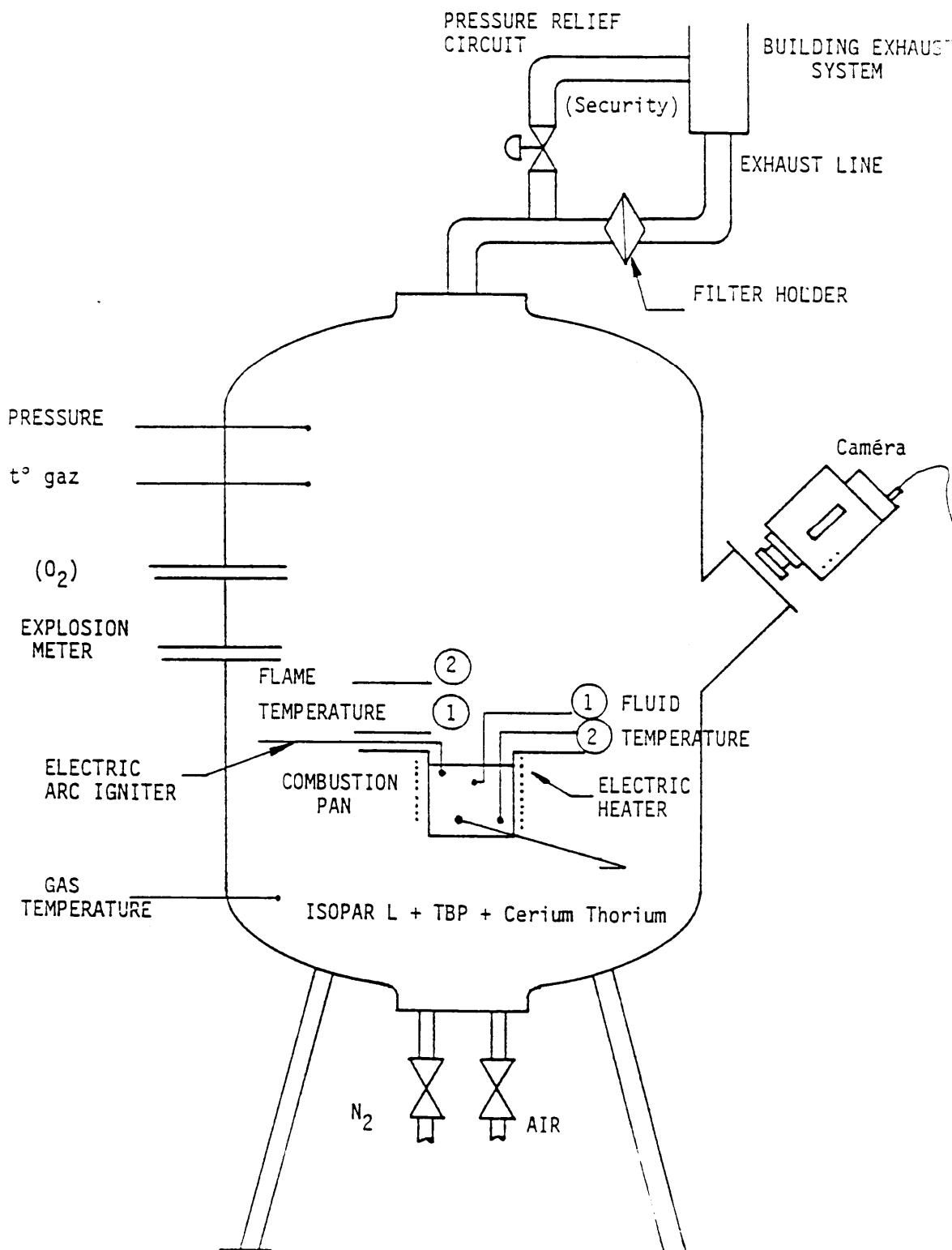
Figure A.11. 316-liter Test Vessel (Figure 1 - Malet Duverger de Cuy, Gasteiger and Janberg April 1983)
