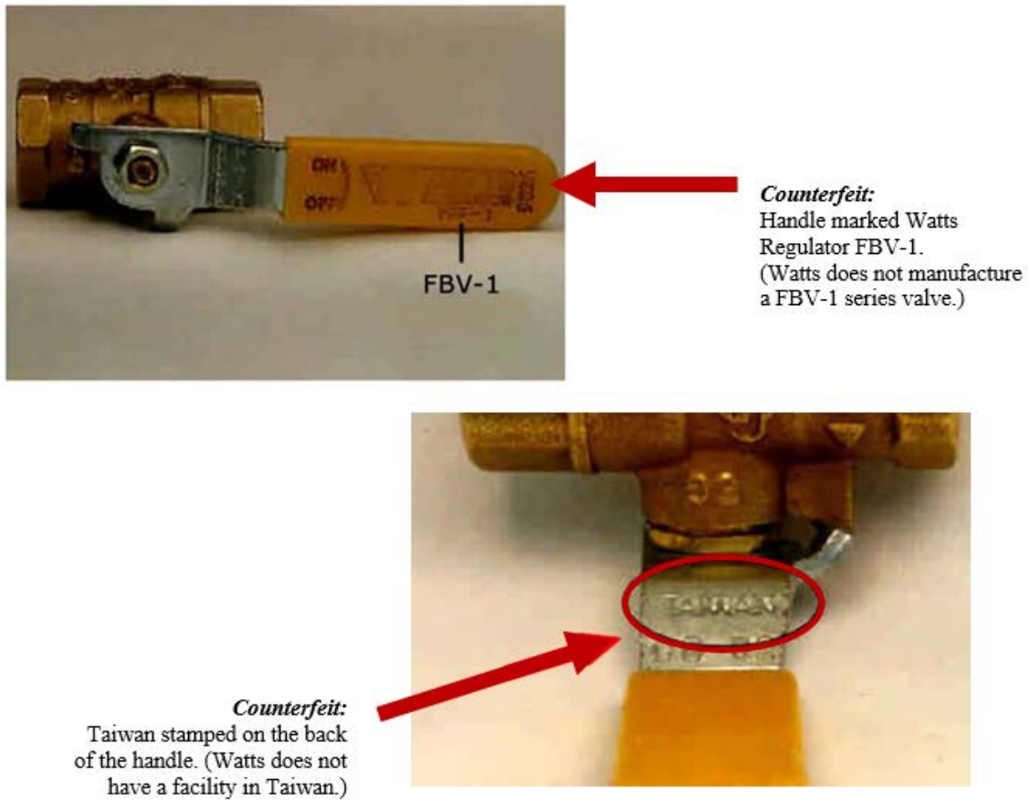
Figure A-8: 1/2" Forged Ball Gas Valves Counterfeit
