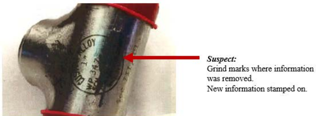
Figure A-22: Stainless Steel “T” Weldalet
