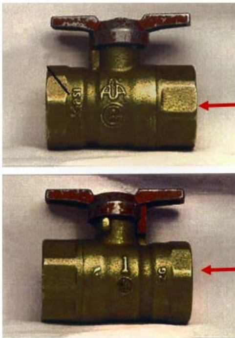
Figure A-13: 1" Forged Ball Gas Valve – Counterfeit
