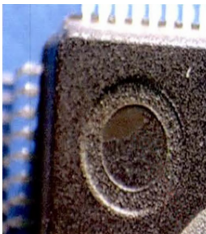
Figure 15: PQFP with Clear Indications of a Blacktop
