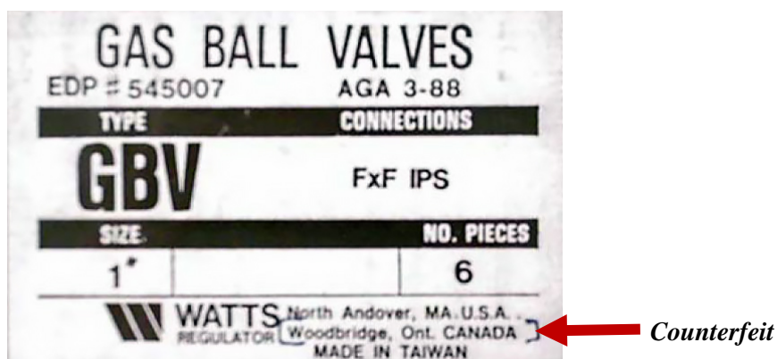
Figure A-2: Suspect WATTS Gas Ball Valve Label
